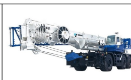
NEW 2019 TADANO GR1200XL (120T) 184' BOOM + 58' JIB
